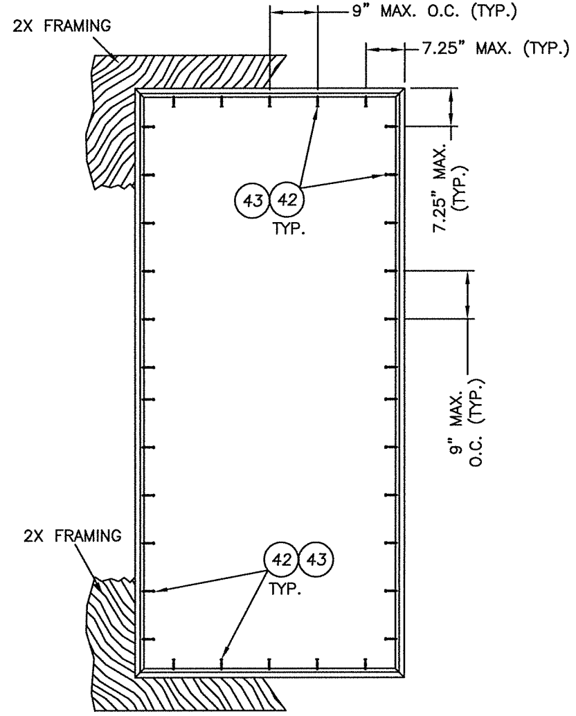
REVEAL MOUNT SUB-FRAME ANCHORING
