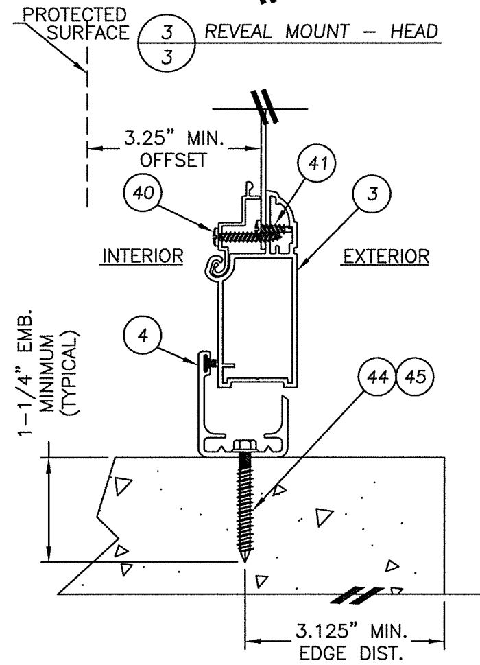
4 REVEAL MOUNT - BASE 3
