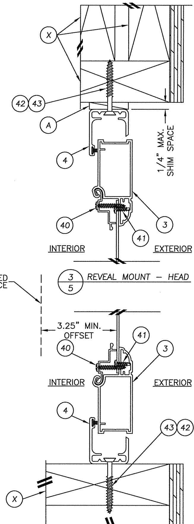
4 REVEAL MOUNT - BASE 5
