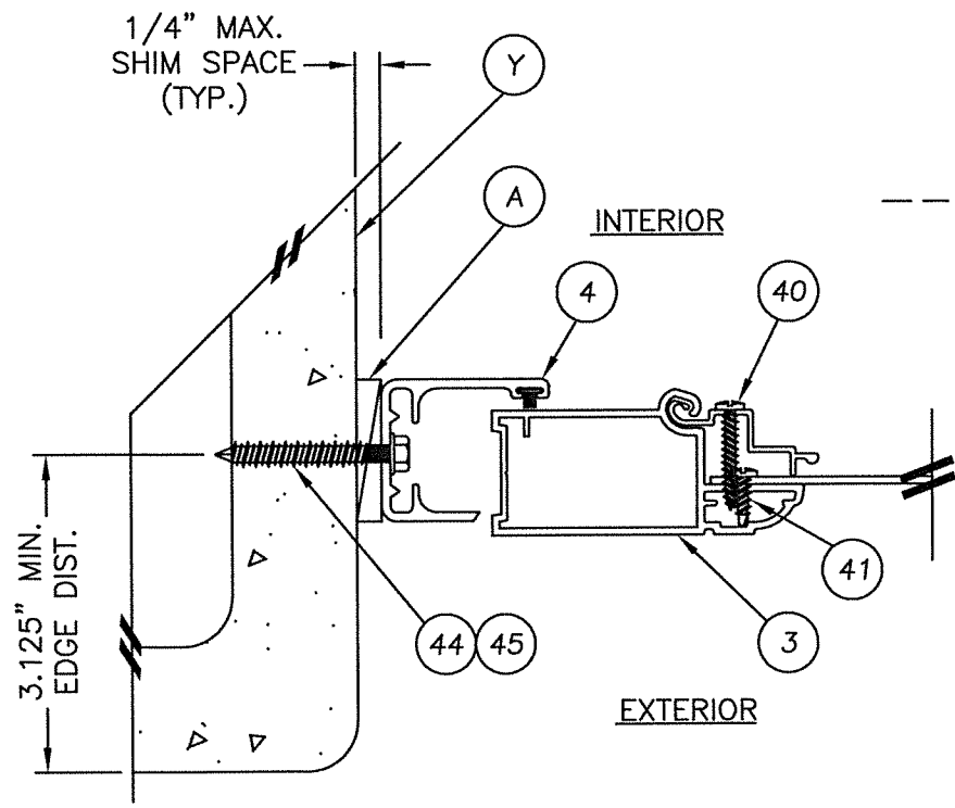
1 REVEAL MOUNT - HINGE JAMB 3 HINGE REMOVED FOR CLARITY
