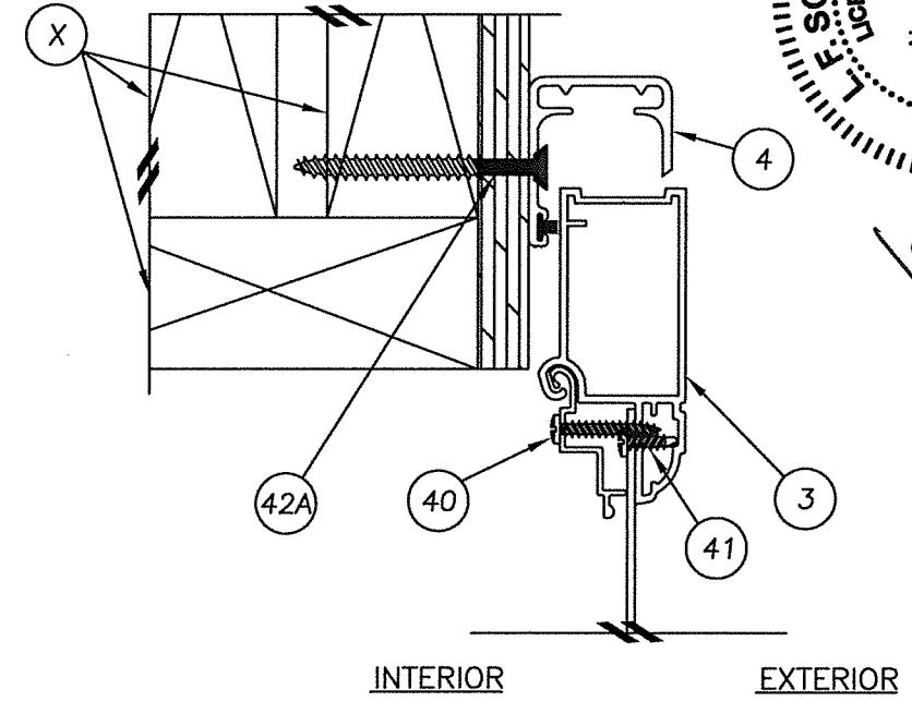
3 SURFACE MOUNT - HEAD 6
