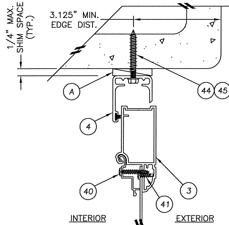
PROTECTED SURFACE 3 REVEAL MOUNT - HEAD 3
