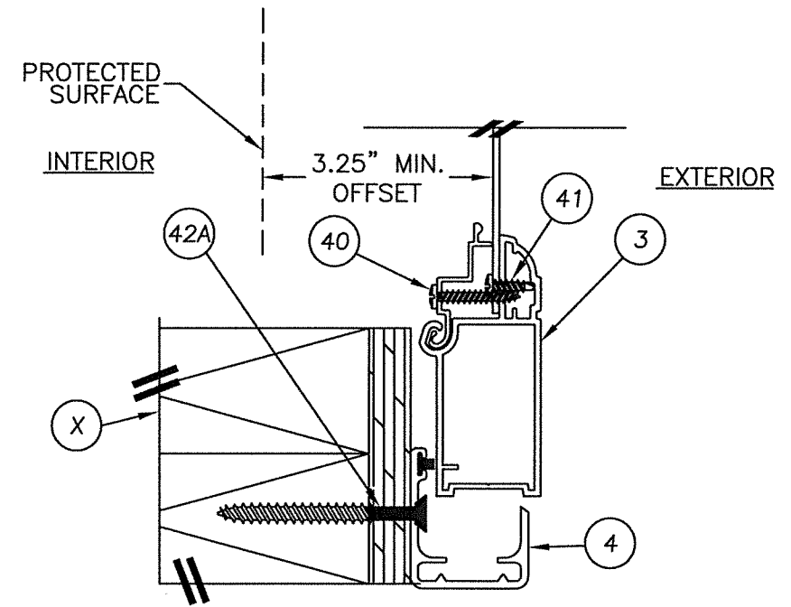
3 SURFACE MOUNT - HEAD 6
